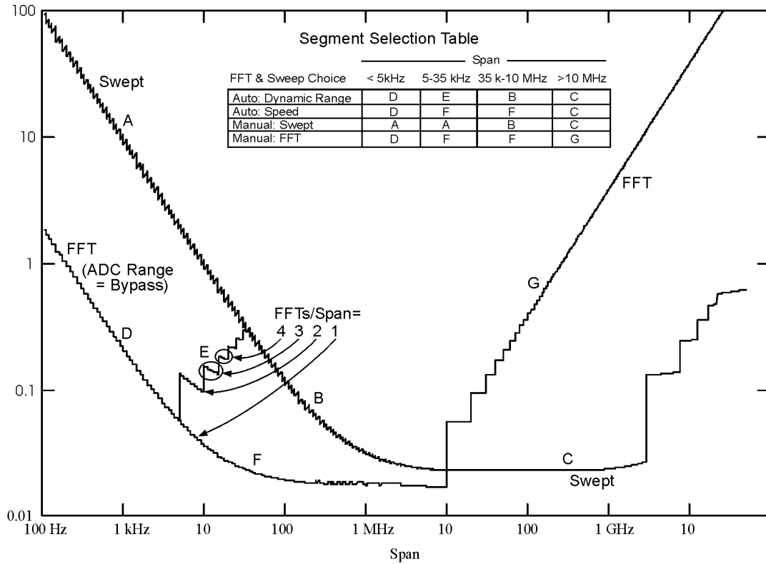
Measurement Time vs. Span (nominal)
