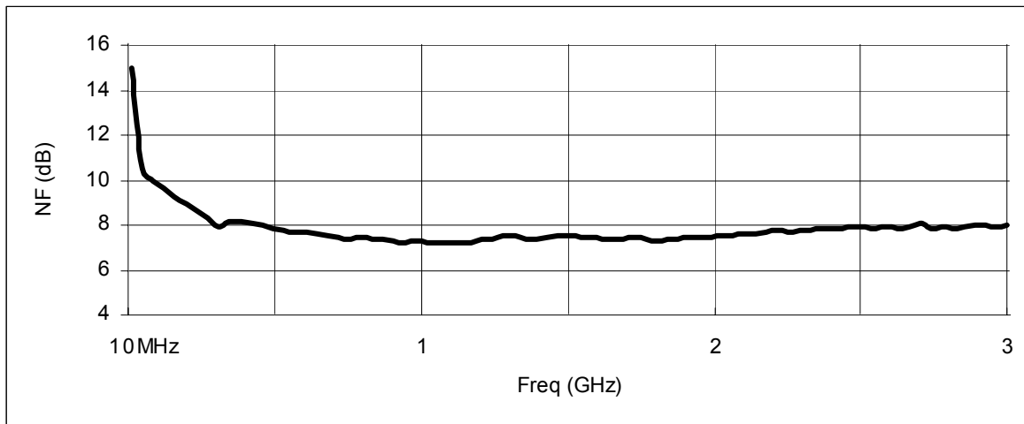
Nominal Instrument Noise Figure 10 MHz to 3 GHz Option 110 Preamp On
