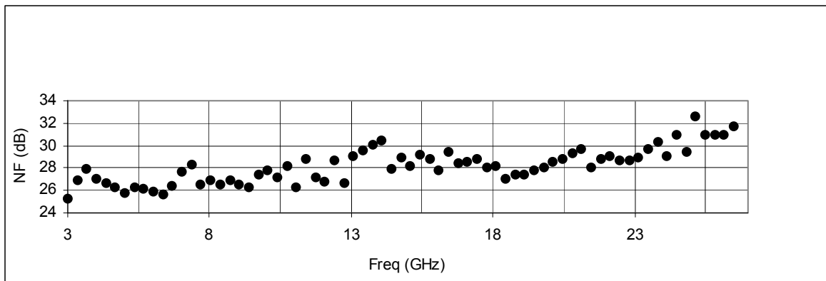
Nominal Instrument Noise Figure 3 to 26.5 GHz No Preamp
