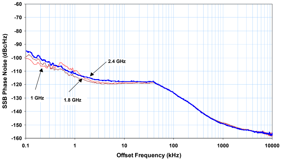
Nominal Phase Noise at Common Cellular Communication Frequencies, \mathcal{L}(f) Optimized Versus f
